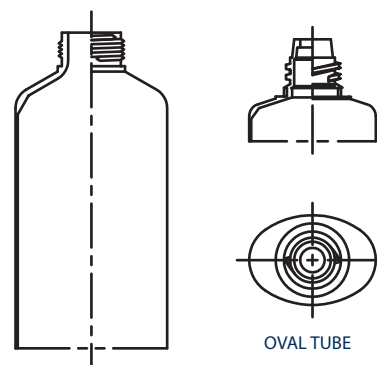
STANDARD HEAD WITH THREAD
